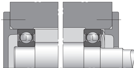
figure 23 The deep groove ball bearing that preloaded by the wave spring
