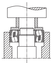
Figure 5: tight fit of outer ring and inner ring
