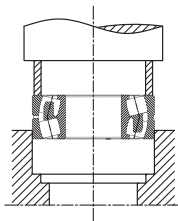
Figure 4: tight fit of outer ring
