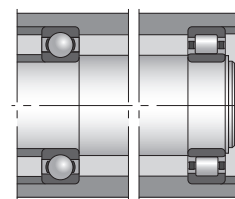
pic2 deep groove ball bearing - cylindrical roller bearing
