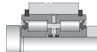
pic 19 SL series bearing
