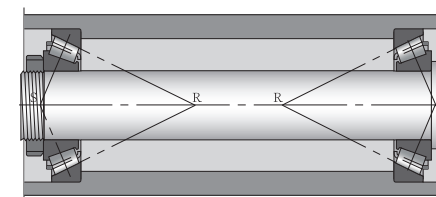
figure11 Tapered ball bearing - Type O configuration
