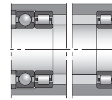
pic6 combined bearing - cylindrical roller bearing
