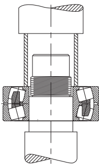
Figure 3: Arbor Press Method
