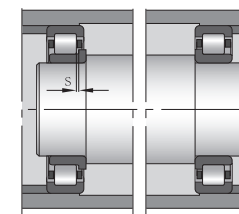
figure14 Cylindrical roller bearing
