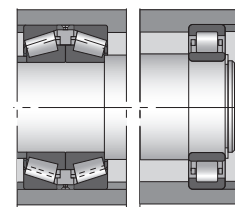
pic5 matched tapered roller bearing - cylindrical roller bearing
