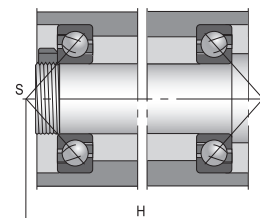
figure8 Angular contact ball bearings - Type O configuration
