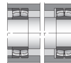
pic7 Double row spherical roller bearing - Double row spherical roller bearing
