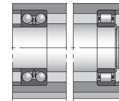
pic4 double row angular contact ball bearings - cylindrical roller bearing
