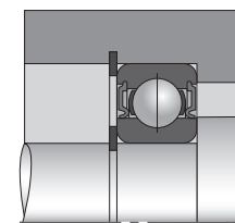
figure16 Deep groove ball bearing
