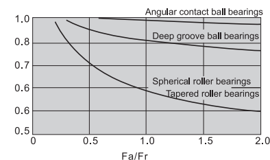
Fig 3: Modification the limit rotation speed according bearing load
