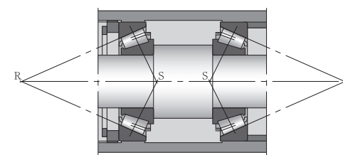
figure10 Tapered ball bearing - Type X configuration
