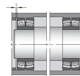
figure13 Double-row spherical roller bearing
