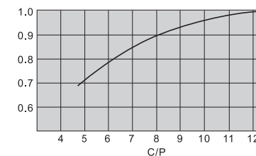
Fig 4: Modification of Limiting Speed under Synthetic Load
