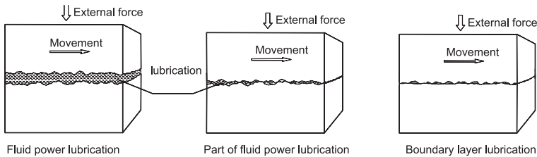
Figure：lubrication mechanism
