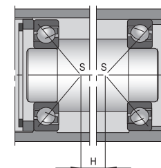
figure9 Angular contact ball bearings - Type X configuration
