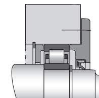
figure22 Cylindrical roller bearing
