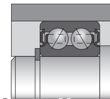
figure21 Double-row angular contact ball bearing
