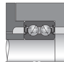
pic-17 Double-row angular contact ball bearing
